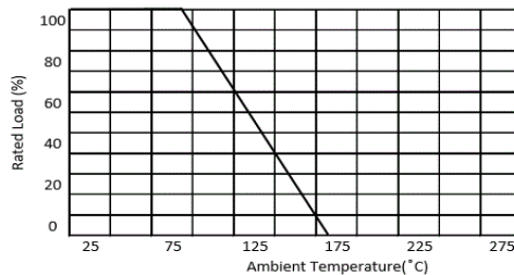
Derating Curve :
