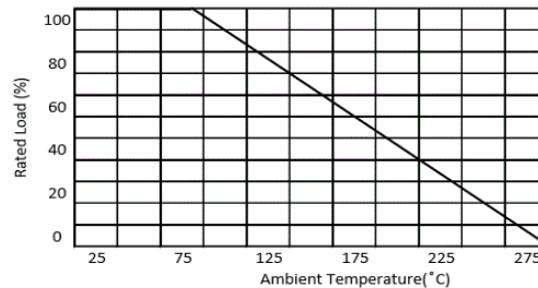
Derating Curve :
